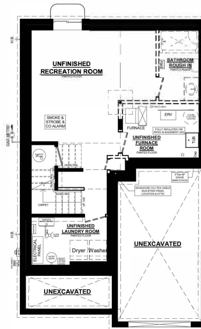
KENSINGTON B UNIT #1 BASEMENT PLAN
