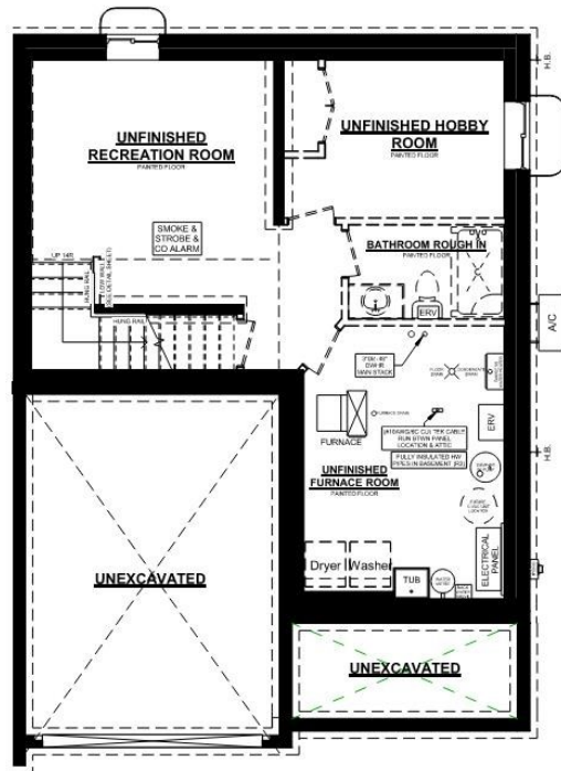
ELMWOOD C UNIT #2 BASEMENT PLAN
