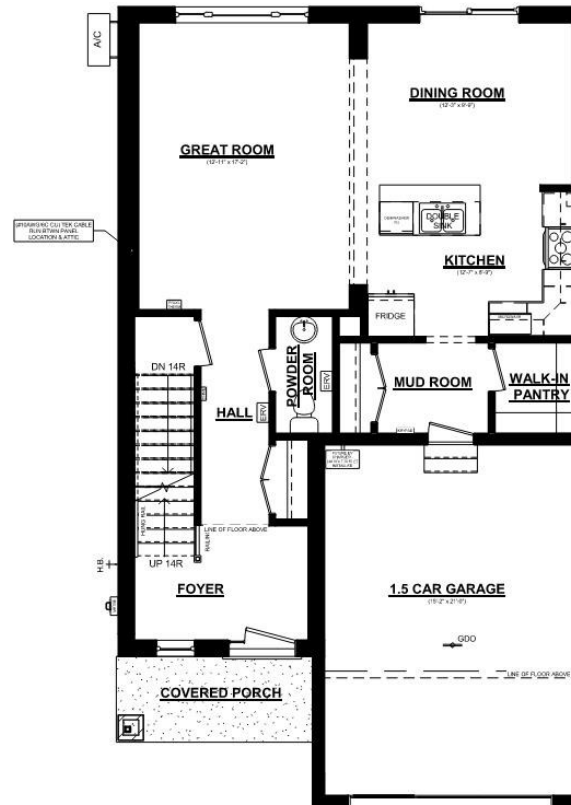
SEDONA 'A' UNIT #1 MAIN FLOOR PLAN 879 SQ. FT. 8' CEILINGS ON MAIN FLOOR
