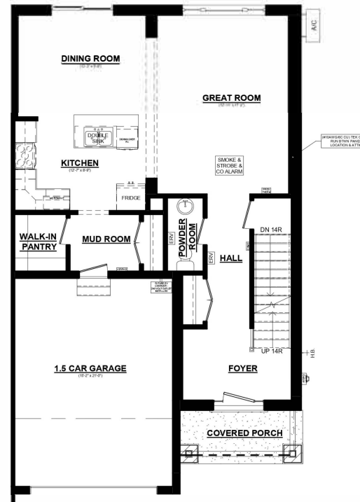
SEDONA 'C' UNIT #2 MAIN FLOOR PLAN 879 SQ. FT. 8\"/>
