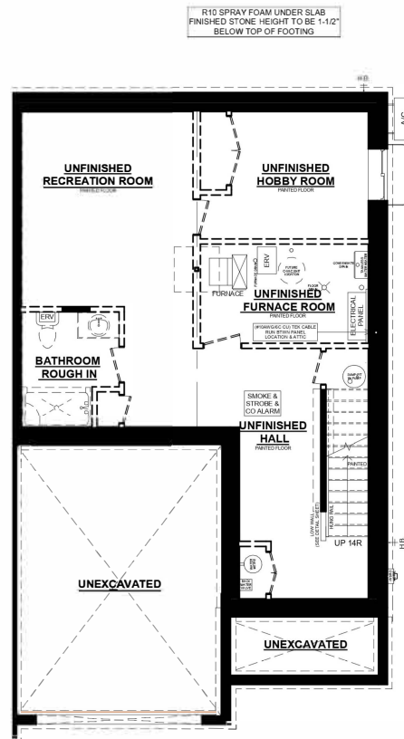
SEDONA 'C' UNIT #1 BASEMENT PLAN
