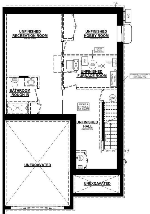
SEDONA 'A' UNIT #2 BASEMENT PLAN
