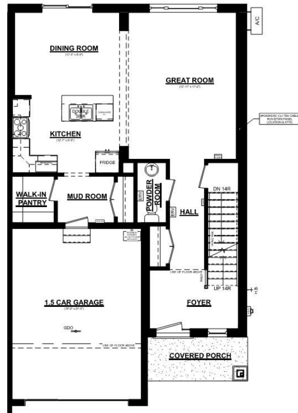
SEDONA 'A' UNIT #2 MAIN FLOOR PLAN 879 SQ. FT. 8' CEILINGS ON MAIN FLOOR
