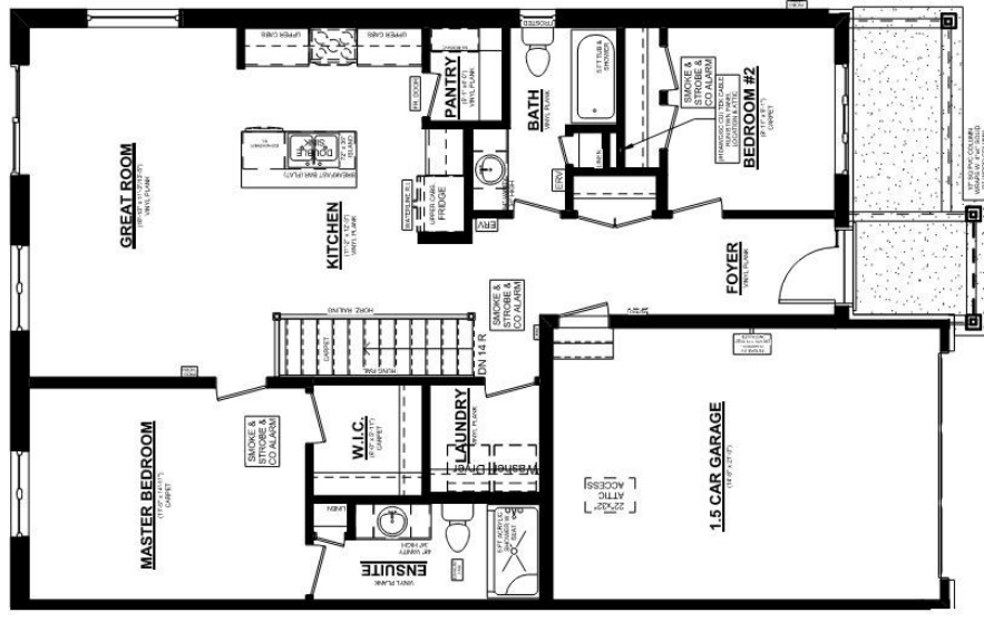
EASTON A UNIT #2 MAINFLOOR PLAN 1200 SQ. FT. 8' CEILINGS ON MAINFLOOR
