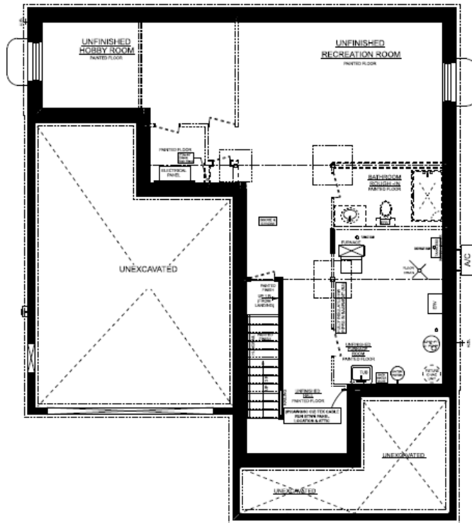
IVYSTONE 'B' BASEMENT PLAN
