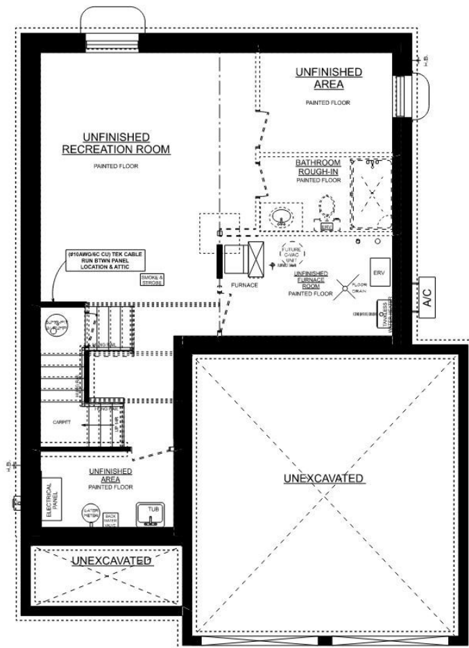
MAPLERIDGE 'A' BASEMENT PLAN UNFINISHED BASEMENT
