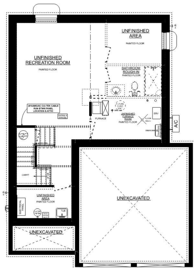
MAPLERIDGE 'A' BASEMENT PLAN UNFINISHED BASEMENT
