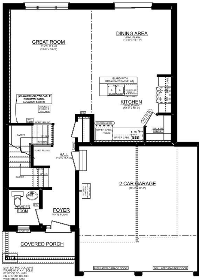
MAPLERIDGE 'A' MAINFLOOR PLAN 797 SQ. FT. 2 CAR 8' CEILINGS ON MAINFLOOR
