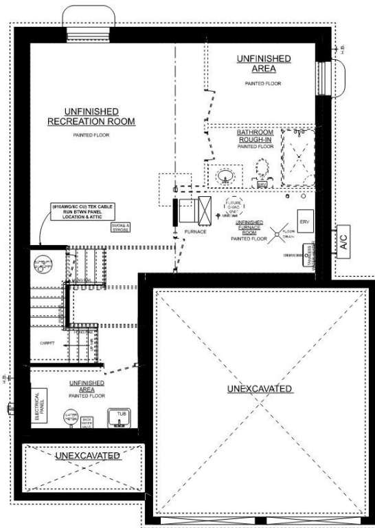
MAPLERIDGE 'A' BASEMENT PLAN UNFINISHED BASEMENT
