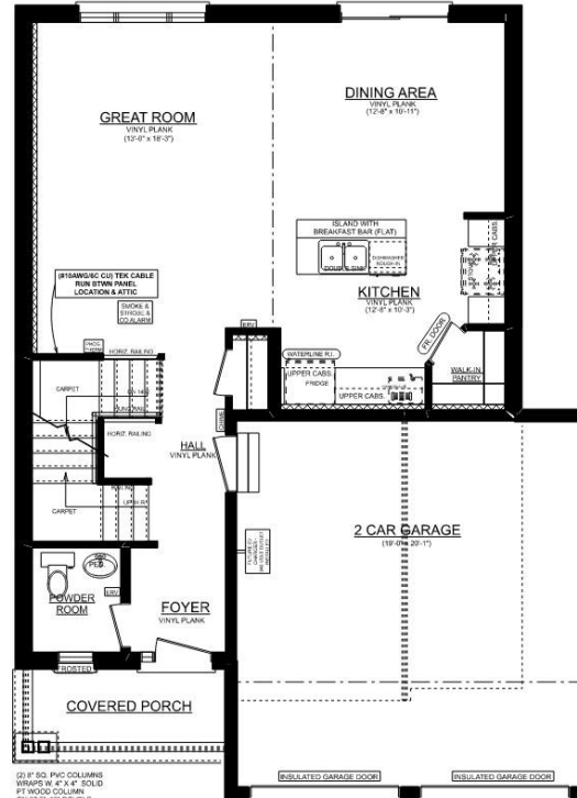
MAPLERIDGE 'A' MAINFLOOR PLAN 797 SQ. FT. 2 CAR 8' CEILINGS ON MAINFLOOR
