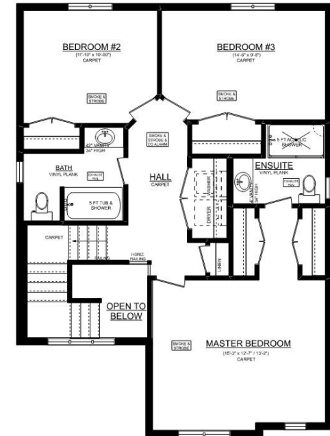
MAPLERIDGE 'A' 2ND FLOOR PLAN 871 SQ. FT. (DOES NOT INCLUDE 95 SQ.FT. OPEN TO BELOW) 8' CEILINGS ON 2ND FLOOR
