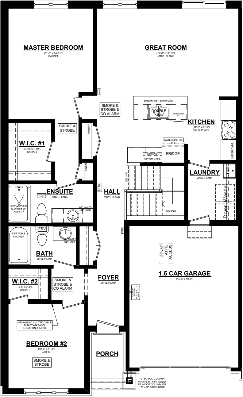
SUTHERLAND A UNIT #1 MAIN FLOOR PLAN 1300 SQ. FT. 8' CEILINGS ON MAIN FLOOR
