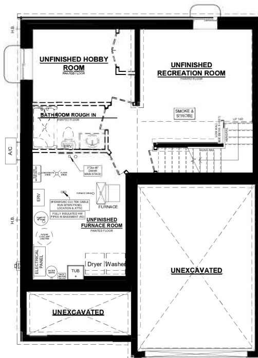
ELMWOOD C UNIT #1 BASEMENT PLAN
