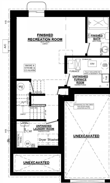
KENSINGTON B UNIT #1 BASEMENT PLAN 310 SQ. FT. FINISHED BASEMENT SPACE
