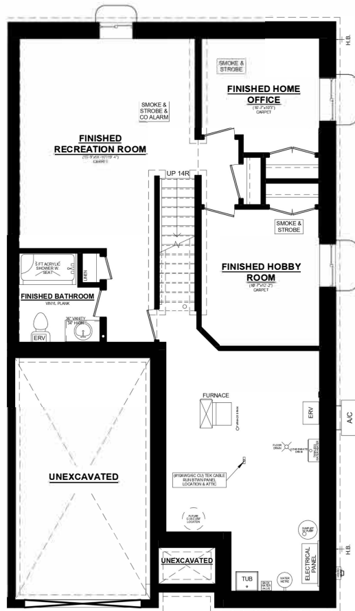
VALLEYBROOK 'C' UNIT #2 BASEMENT PLAN 615 SQ. FT. FINISHED BASEMENT SPACE
