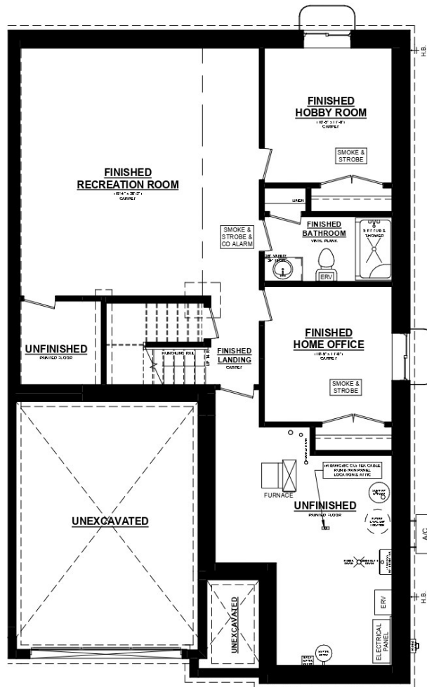
SUTHERLAND A UNIT #2 BASEMENT PLAN
