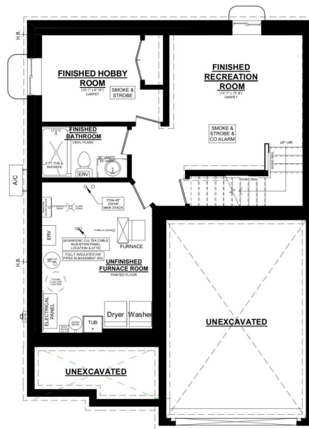
ELMWOOD B UNIT #1 BASEMENT PLAN
