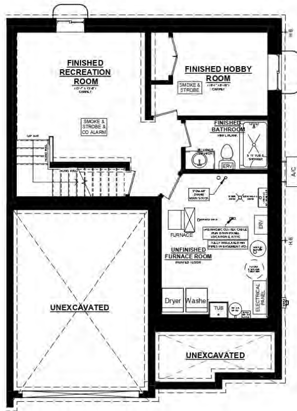
ELMWOOD B UNIT #2 BASEMENT PLAN
