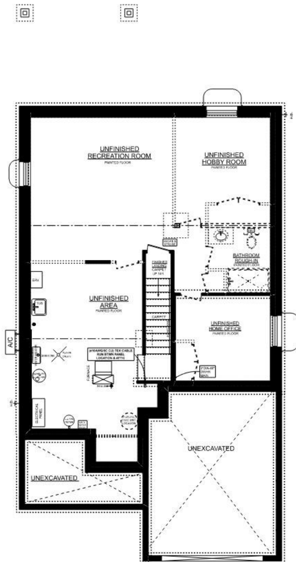
MAYFAIR 'B' BASEMENT PLAN UNFINISHED BASEMENT
