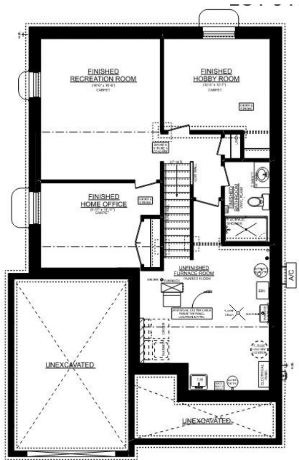
PINEWOOD 'B' BASEMENT PLAN 626 SQ. FT. FINISHED BASEMENT
