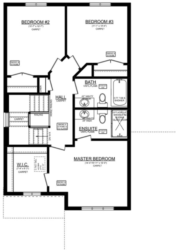
ASPEN 'B' 2ND FLOOR PLAN 775 SQ. FT. (DOES NOT INCLUDE 65 SQ. FT. OPEN TO BELOW) 8' CEILINGS ON 2ND FLOOR
