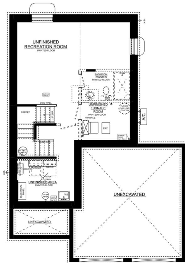
ASPEN 'B' BASEMENT PLAN 2 CAR
