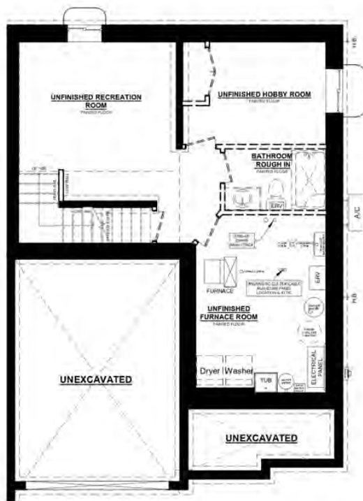
ELMWOOD B UNIT #2 BASEMENT PLAN
