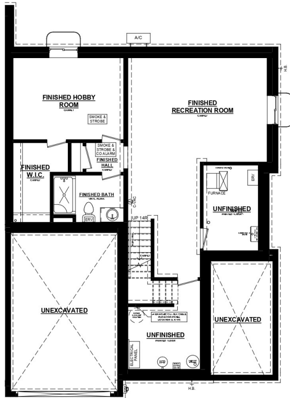
ROCKWOOD B UNIT #2 BASEMENT PLAN 686 SQ. FT. FINISHED BASEMENT SPACE
