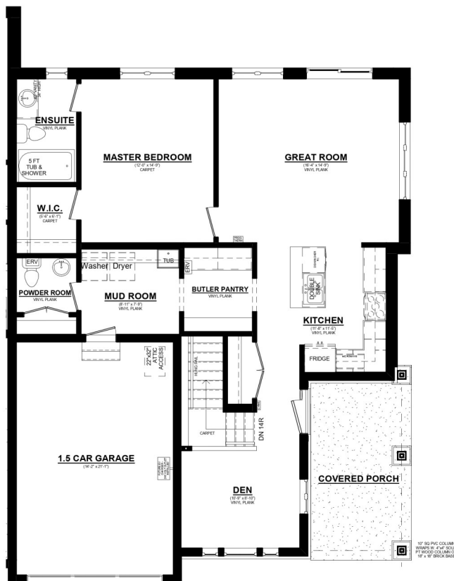
ROCKWOOD B UNIT #2 MAIN FLOOR PLAN 1130 SQ. FT. 8' CEILINGS ON MAIN FLOOR
