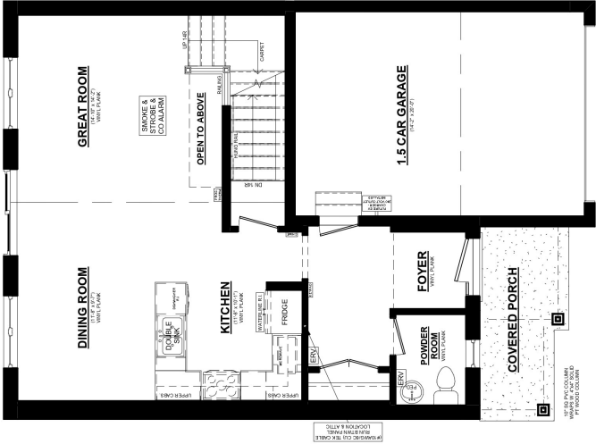
ELMWOOD B UNIT #1 MAINFLOOR PLAN 745 SQ. FT. 8' CEILINGS ON MAINFLOOR
