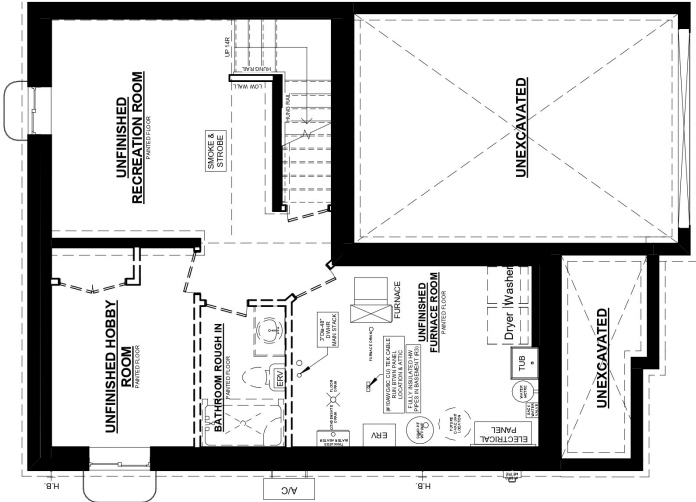
ELMWOOD B UNIT #1 BASEMENT PLAN
