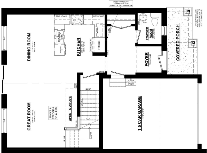
ELMWOOD B UNIT #2 MAINFLOOR PLAN 745 SQ. FT. 8' CEILINGS ON MAINFLOOR
