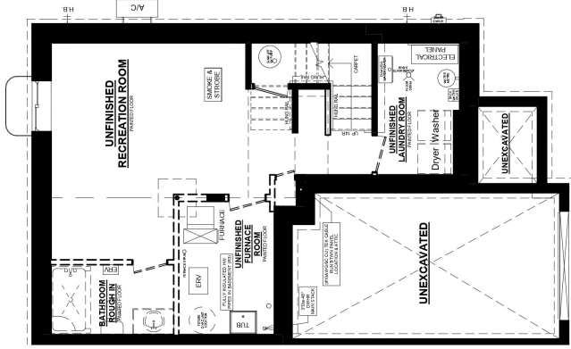
KENSINGTON C UNIT #2 BASEMENT PLAN
