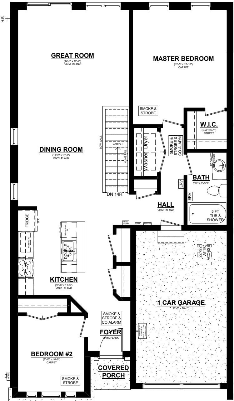
VALLEYBROOK D UNIT #1 MAIN FLOOR PLAN 1185 SQ. FT. 8' CEILINGS ON MAIN FLOOR
