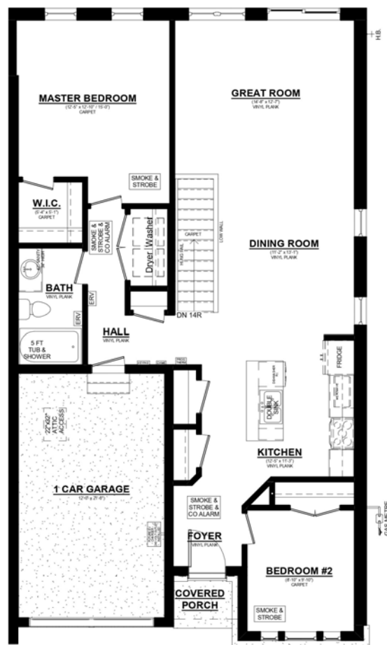
VALLEYBROOK D UNIT #2 MAIN FLOOR PLAN 1185 SQ. FT. 8" CEILINGS ON MAIN FLOOR
