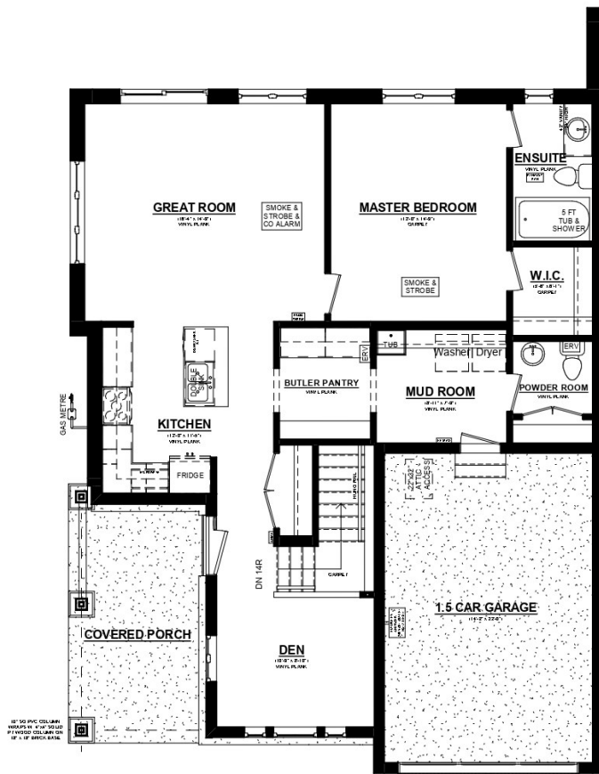
ROCKWOOD B UNIT #1 MAIN FLOOR PLAN 1066 SQ. FT. 8" CEILINGS ON MAIN FLOOR
