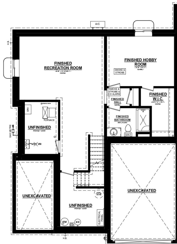
ROCKWOOD B UNIT #1 FINISHED BASEMENT PLAN 686 SQ. FT. FINISHED FINISHED BASEMENT SPACE
