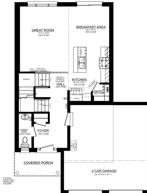
ASPEN 'B' MAINFLOOR PLAN 8' CEILINGS ON MAINFLOOR 700 SQ. FT. 2 CAR GARAGE
