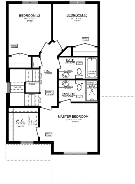
ASPEN 'B' 2ND FLOOR PLAN 775 SQ. FT. (DOES NOT INCLUDE 65 SQ. FT. OPEN TO BELOW) 8' CEILINGS ON 2ND FLOOR
