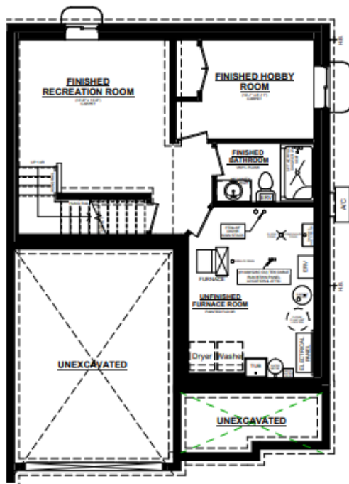
ELMWOOD B UNIT #2 BASEMENT PLAN 433 SQ. FT. FINISHED BASEMENT SPACE
