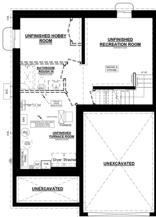
ELMWOOD C UNIT #1 BASEMENT PLAN
