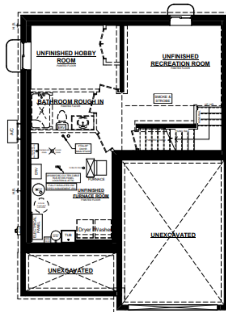
ELMWOOD A UNIT #1 BASEMENT PLAN
