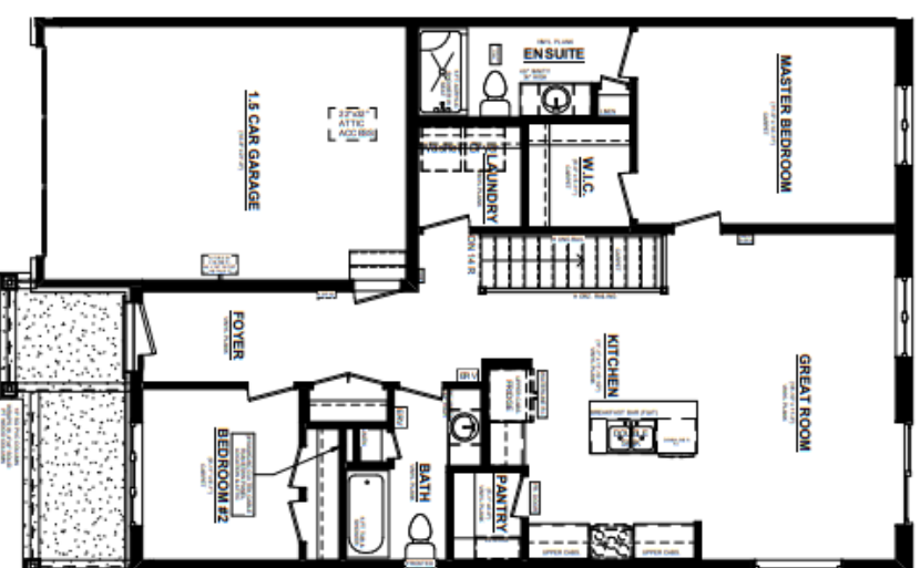
EASTON A UNIT #2 MAINFLOOR PLAN 1200 SQ. FT. 8' CEILINGS ON MAINFLOOR
