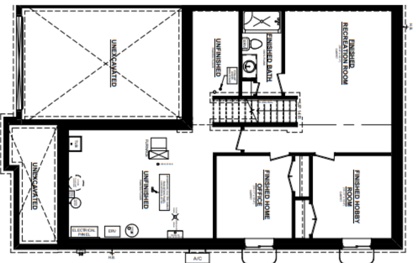
EASTON A UNIT #2 BASEMENT PLAN 605 SQ. FT. FINISHED BASEMENT SPACE
