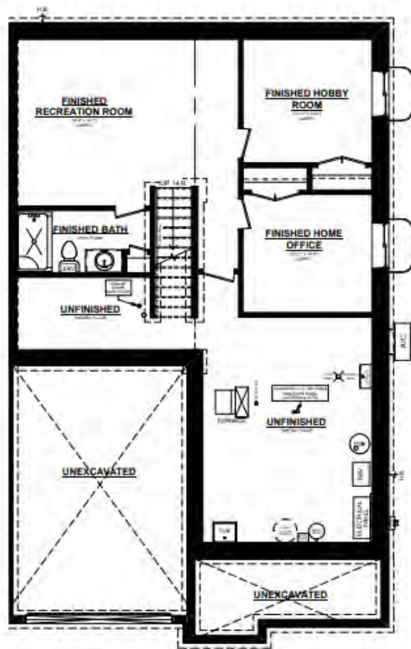
EASTON A UNIT #2 BASEMENT PLAN 605 SQ. FT. FINISHED BASEMENT SPACE
