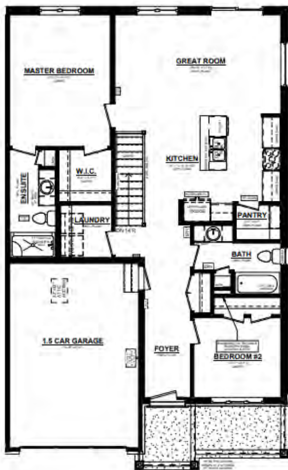
EASTON A UNIT #2 MAIN FLOOR PLAN 1200 SQ. FT. 8" CEILINGS ON MAIN FLOOR
