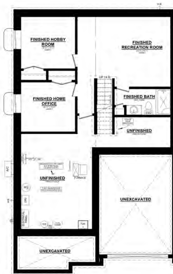
EASTON A UNIT #1 BASEMENT PLAN 605 SQ. FT. FINISHED BASEMENT SPACE
