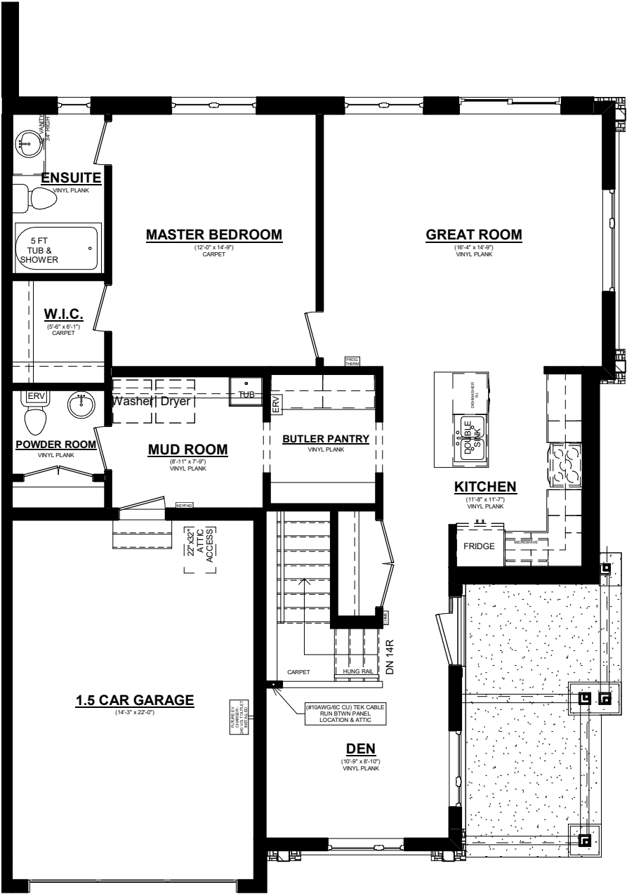
ROCKWOOD A UNIT #2 MAIN FLOOR PLAN 651 SQ. FT. 8' CEILINGS ON MAIN FLOOR
