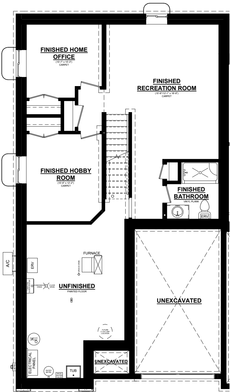
VALLEYBROOK A UNIT #1 BASEMENT PLAN 663 SQ. FT. FINISHED BASEMENT SPACE
