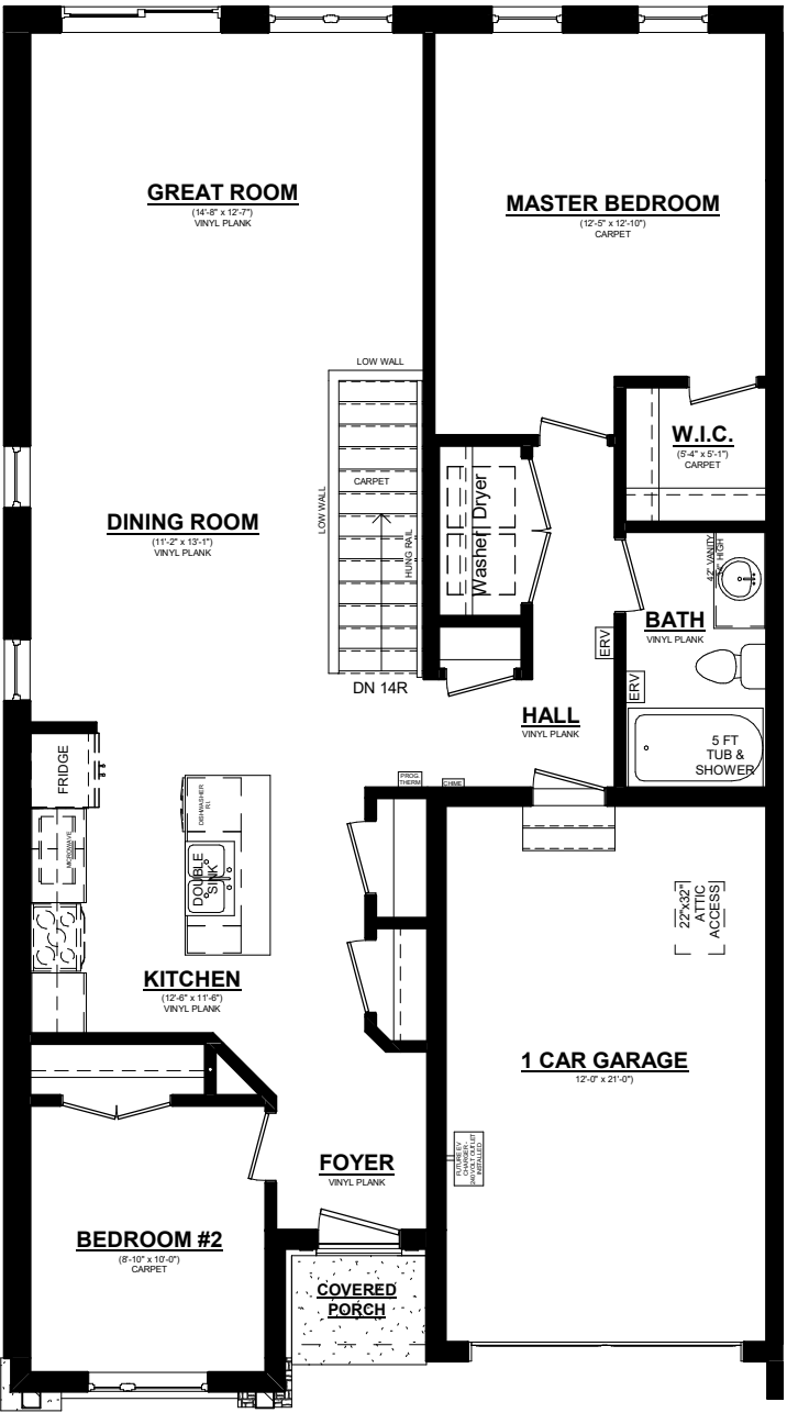
VALLEYBROOK A UNIT #1 MAIN FLOOR PLAN 1185 SQ. FT. 8' CEILINGS ON MAIN FLOOR
