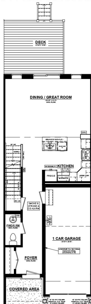
ASHTON 'C' UNIT #3 LOT #14 EMPIRE PARKWAY
