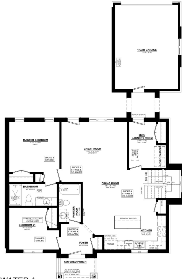
BRIDGEWATER A MAIN FLOOR PLAN 1288 SQ. FT. 8' CEILINGS ON MAINFLOOR PUBLISHER
