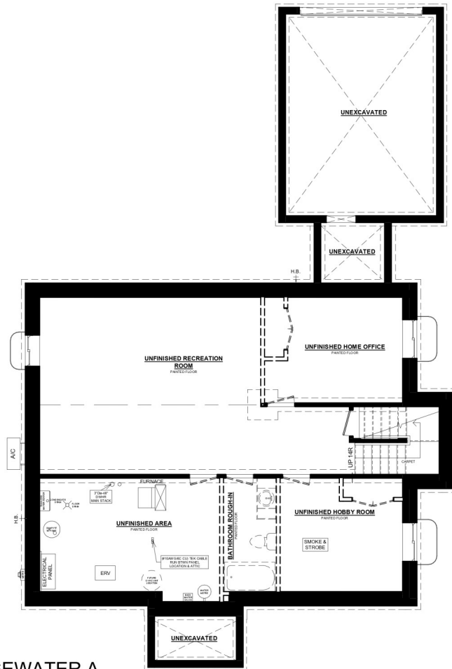
BRIDGEWATER A UNFINISHED BASEMENT PLAN
