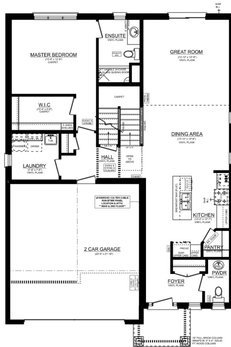
THE STONEHAVEN 'B' MAINFLOOR PLAN 1313 SQ. FT. 8' CEILINGS ON MAIN FLOOR
