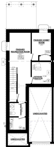
Ashton B UNIT #1 BASEMENT PLAN 378 SQ. FT. FINISHED BASEMENT SPACE
