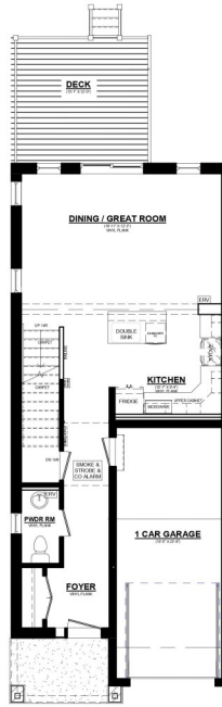
Ashton B UNIT #1 MAINFLOOR PLAN 690 SQ. FT. 8' CEILINGS ON MAINFLOOR' CEILINGS ON MAINFLOOR
