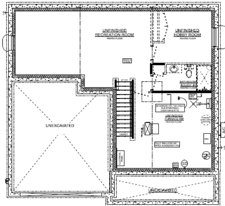
BRIARWOOD 'C' BASEMENT PLAN
