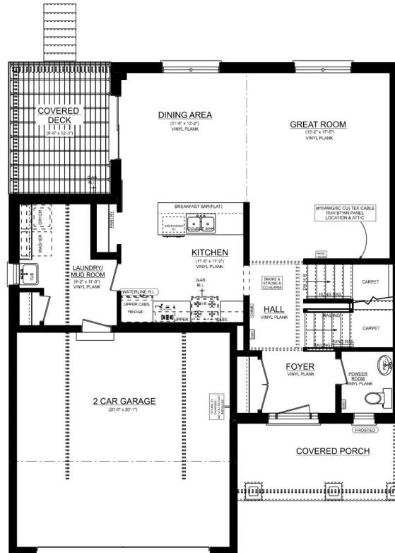
BROOKSTONE 'C' MAIN FLOOR PLAN 945 SQ.FT. 8' CEILINGS ON MAIN FLOOR
