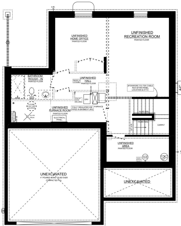
BROOKSTONE 'C' BASEMENT PLAN
