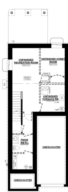
Ashton B UNIT #1 BASEMENT PLAN
