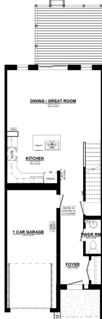
Ashton B MAINFLOOR PLAN 660 SQ. FT. 8" CEILINGS ON MAINFLOOR
