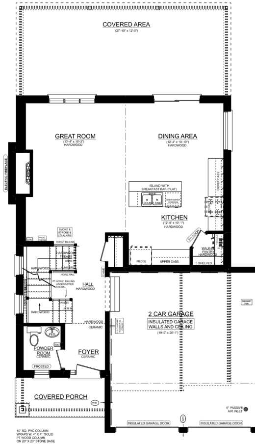
MAPLERIDGE 'A' MAINFLOOR PLAN 9' CEILINGS ON MAINFLOOR 799 SQ. FT. 2 CAR
