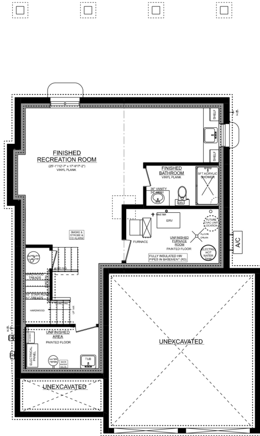
MAPLERIDGE 'A' BASEMENT PLAN 455 SQ. FT. FINISHED SPACE
