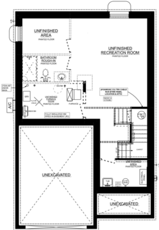
MAPLERIDGE 'A' BASEMENT PLAN
