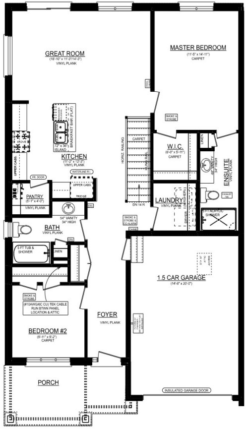
EASTON 'A' UNIT #1 MAIN FLOOR PLAN 1200 SQ. FT. 8' CEILINGS ON MAINFLOOR
