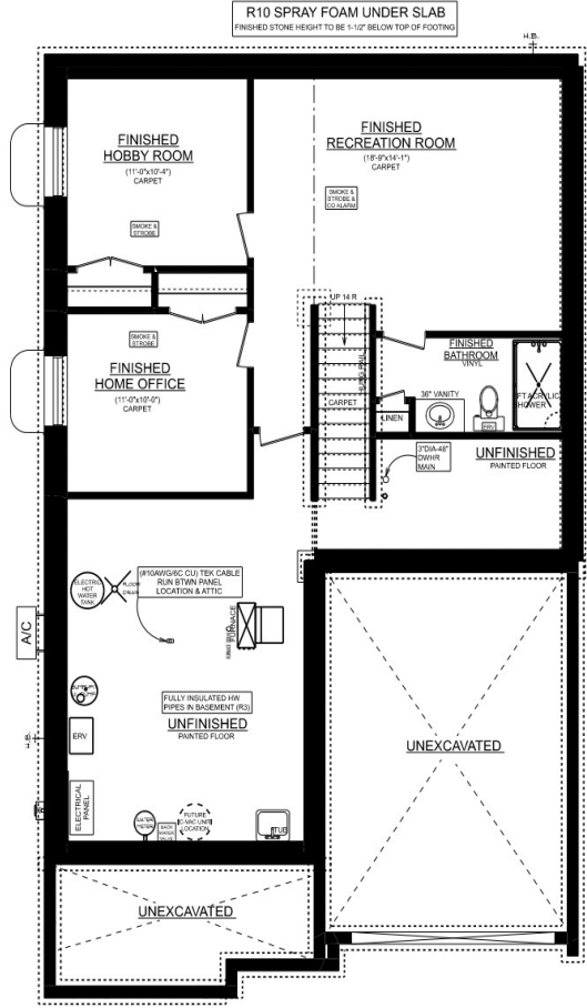
EASTON 'A' UNIT #1 BASEMENT PLAN 592 SQ. FT. FINISHED BASEMENT SPACE
