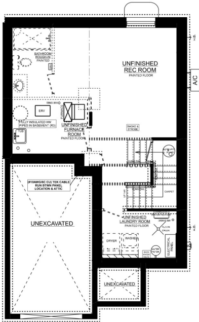
KENSINGTON 'C' UNIT #2 BASEMENT PLAN
