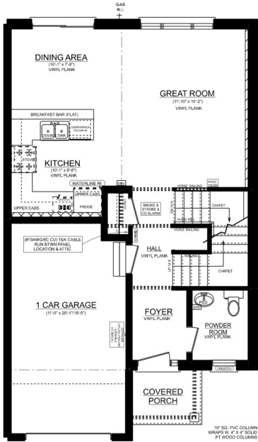
KENSINGTON 'C' UNIT #2 MAIN FLOOR PLAN 8' CEILINGS ON MAIN FLOOR 1 CAR 650 SQ. FT.
