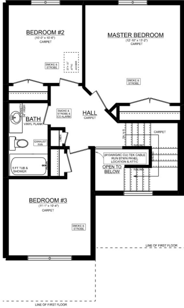
KENSINGTON 'C' UNIT #2 2ND FLOOR PLAN 8' CEILINGS ON 2ND FLOOR 644 SQ. FT. (DOES NOT INCLUDE 87 SQ.FT. OPEN TO BELOW)
