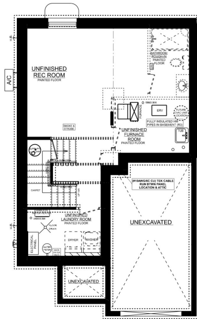
KENSINGTON 'C' UNIT #1 BASEMENT PLAN
