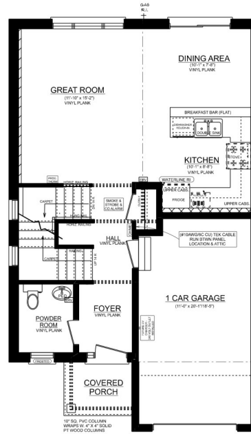
KENSINGTON 'C' UNIT #1 MAINFLOOR PLAN 8' CEILINGS ON MAIN FLOOR 1 CAR 650 SQ. FT.
